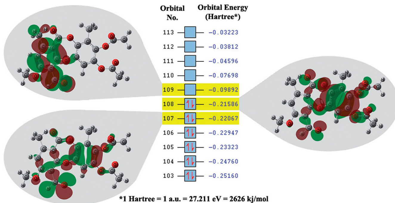
Figure 2. Frontier molecular maps of the depsidone 1 calculated at M06-L/6-31 + G(d,p) level.
