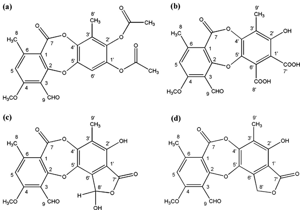
Figure 1. (a) Depsidone 1; (b) Depsidone 2; (c) Stictic acid 3; and (d) Deoxystictic acid 4.
