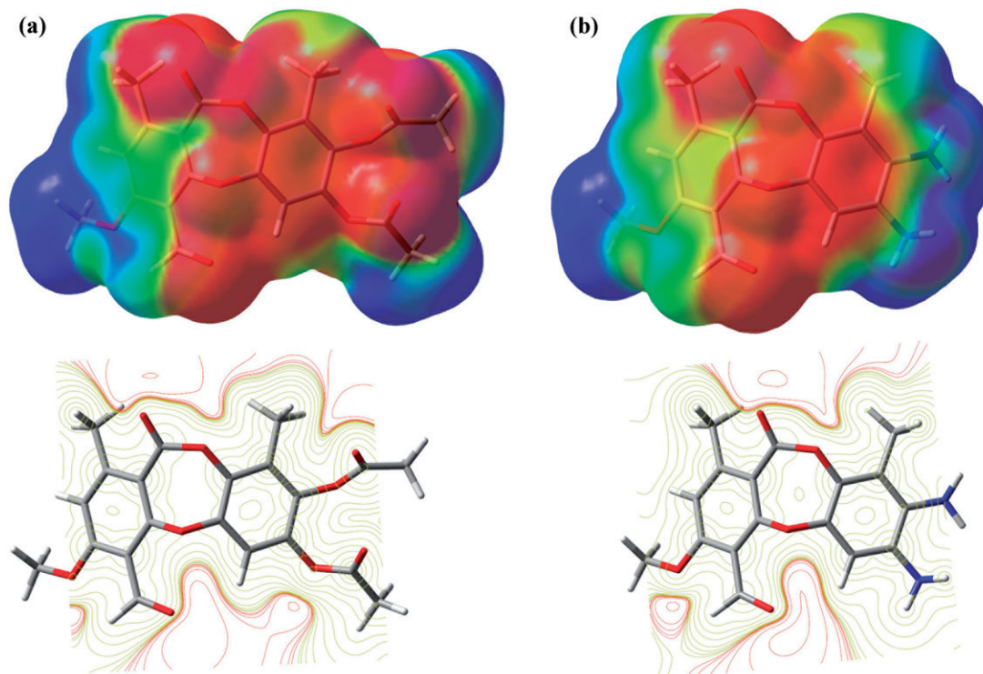
Figure 3. Molecular electrostatic potential (top) and counter (bottom) maps of the depsidone 1 (a) and depsidone 7 (b), calculated at M06-L/6-31+G(d,p) level.
