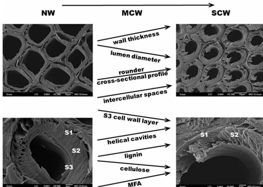
Fig. 2. Scheme for changes in degree of development of tracheid cell wall features characterizing the transition from normal wood (NW) to severe compression wood (SCW), mild compression wood (MCW) forming a continuum between NW and SCW; on the left – field emission scanning electron microscopy (FESEM) images of NW, on the right – FESEM images of SCW; NW – normal wood, MCW - mild compression wood, SCW - severe compression wood, S1, S2, S3 – layers of secondary cell wall
