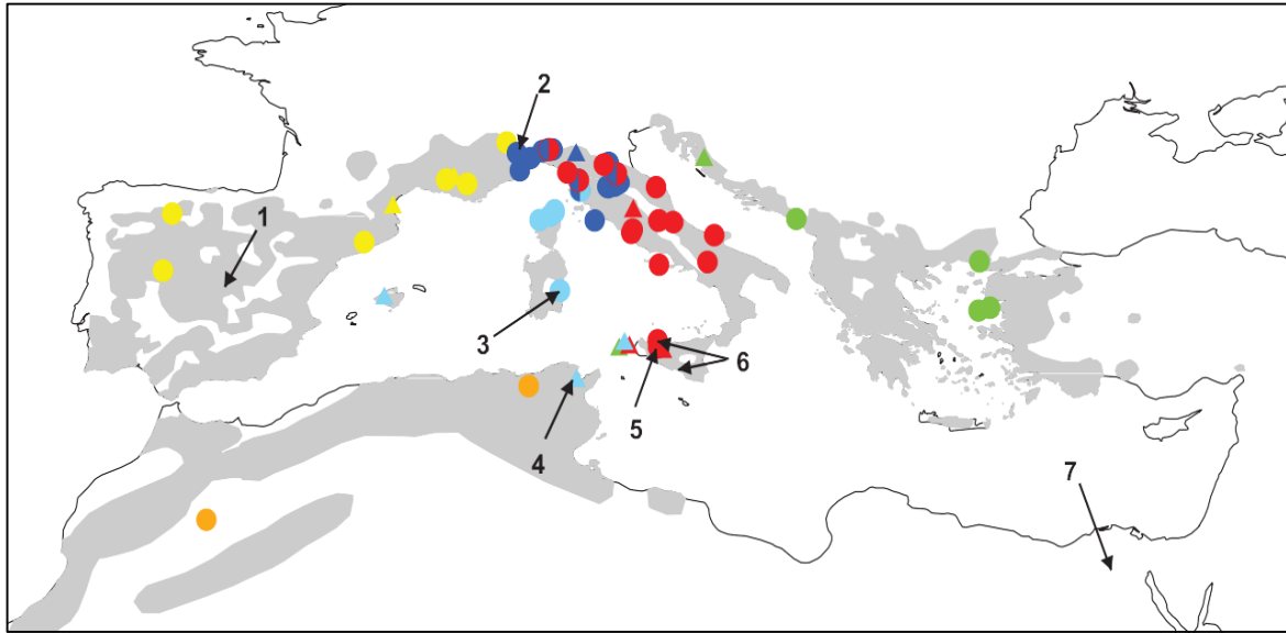
Figure 2. Breeding range of the subalpine warbler Sylvia cantillans complex and origin of samples used in the phylogenetic analysis. The colour code matches the clades recovered in the mitochondrial tree (dots, breeding specimens; triangles, status unknown or migrants; bicoloured dots, localities where specimens of two clades were recorded in syntopy). Collection localities of types are indicated by arrows and numbers: 1, Sylvia inornata iberiae ; 2, Sylvia subalpina ; 3, Sylvia cantillans moltonii ; 4, Sylvia subalpina inornata ; 5, Motacilla cantillans ; 6, Sylvia leucopogon ; 7, Currucula albistriata (approximate). The species range shapefile has been supplied by BirdLife International and Handbook of the Birds of the World (2018) .
